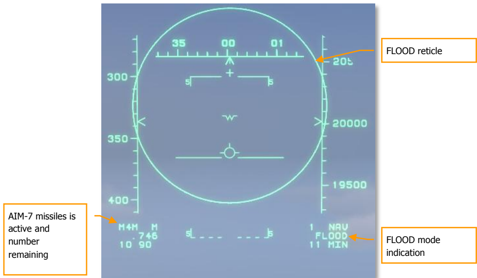
Figure 46. FLOOD mode
