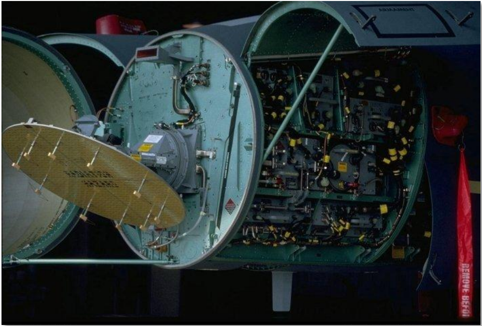
Figure 53. AN/APG-63 radar
