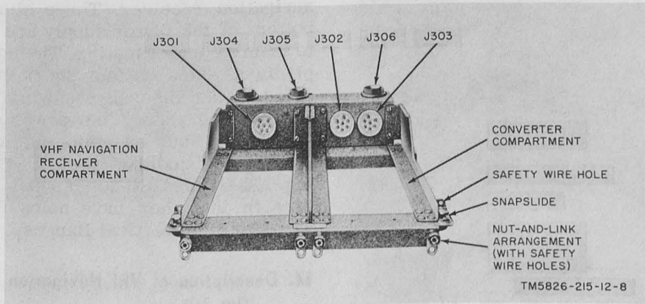
Figure 8. Rack.
