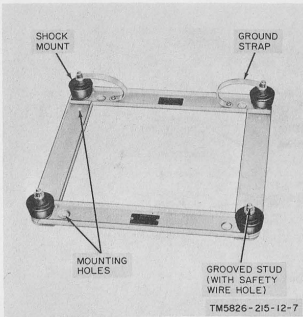
Figure 7. Mounting.
