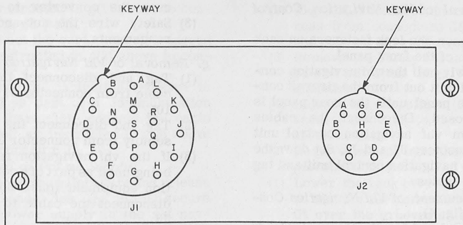
Figure 19. Vhf navigation control unit connectors.
