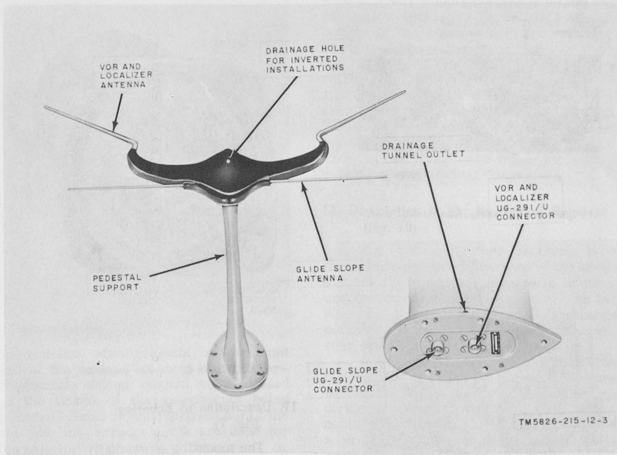
Figure 3. Antenna.
