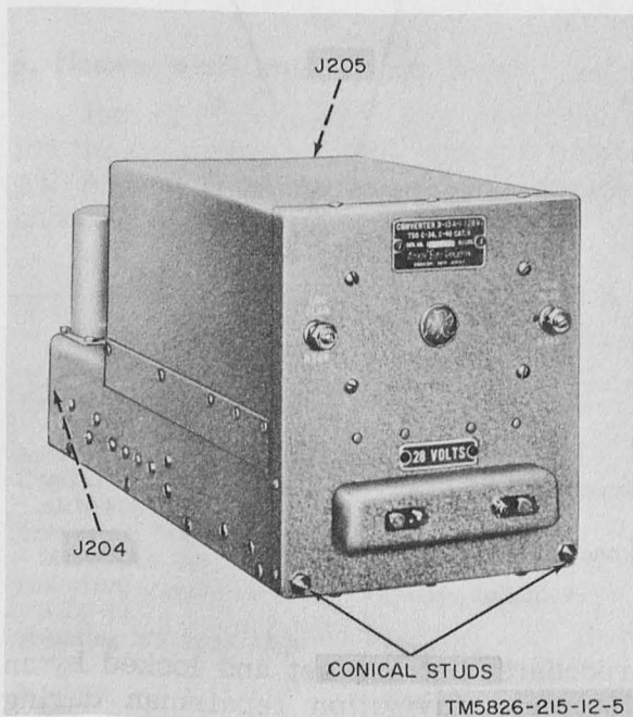
Figure 5. Converter.
