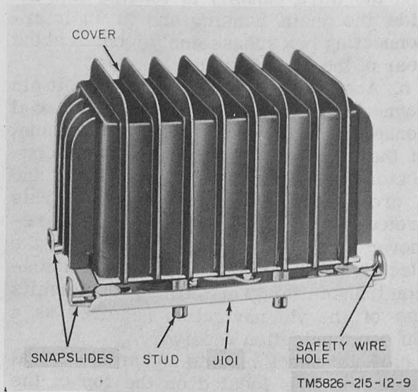
Figure 9. Power supply.
