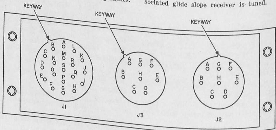
Figure 19.1. Control, Radio Set C-3436A/ARN-30E, electrical connectors.
