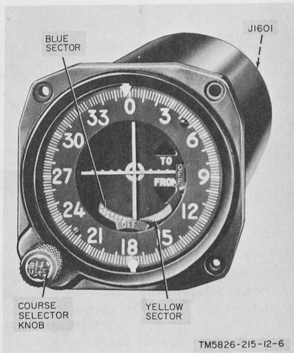
Figure 6. Course indicator.
