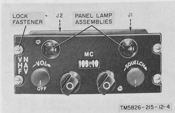
Figure 4. Vhf navigation control unit.
